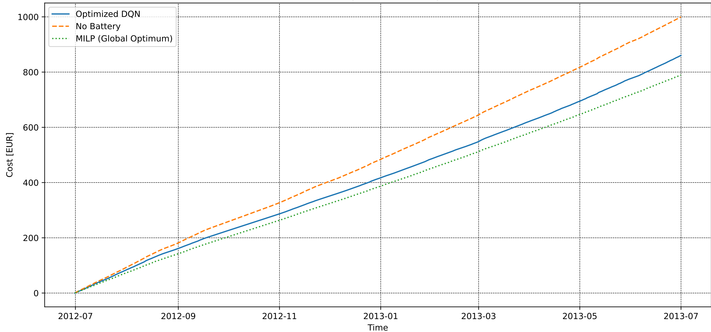
User 66 - Extended Convergence - Electricity Cost [DQN vs MILP]
